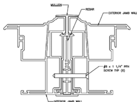
Series 151 Mullion Assembly:
